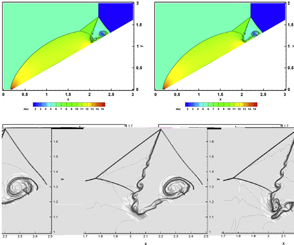
Fig. 11. Results obtained for the Double Mach Reflection Problem at t = 0.21 with the P_0P_2 scheme. A mesh with h = 1/800 has been used. Left column: the new unstructured FORCE flux. Right column: the classical Rusanov flux.
