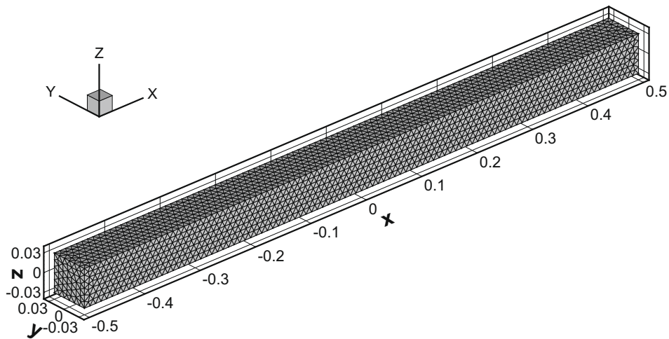
Fig. 5. Unstructured tetrahedral mesh used for the 3D shock tube problems.
