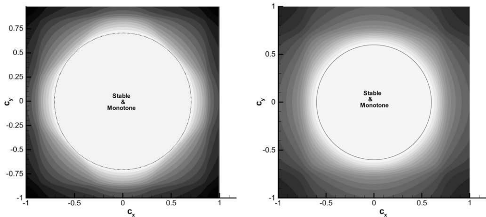
Fig. 12. Linear stability regions for the multi-dimensional FORCE schemes. Left picture depicts the two-dimensional case in the c_x - c_y plane. The right picture shows a cut through the stability region in the c_x - c_y plane for the three-dimensional case.
