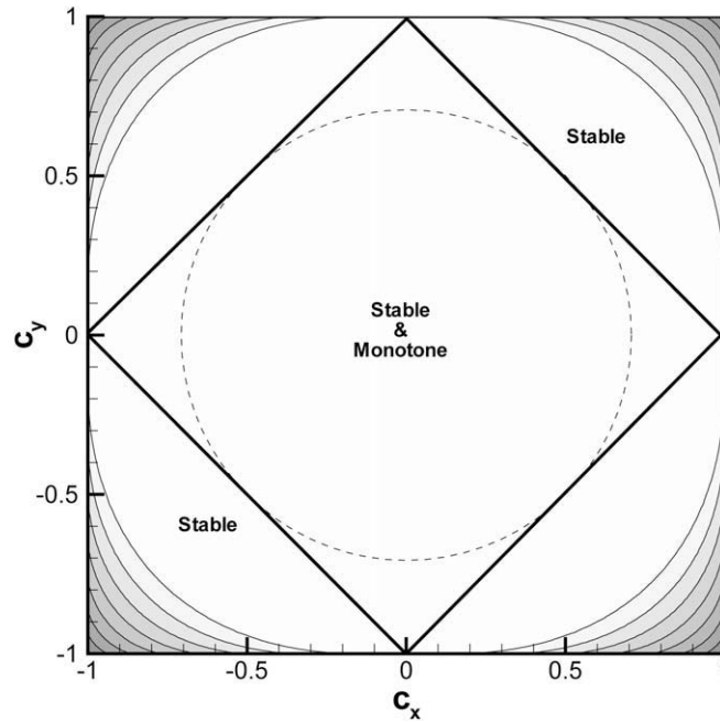
Fig. 13. Linear stability and monotonicity regions for the two-dimensional FORCE scheme on vertex-based secondary volumes (square in full line). Also shown are the stability and monotonicity regions for the two-dimensional FORCE scheme on edge-based secondary volumes (circle in dotted line).
