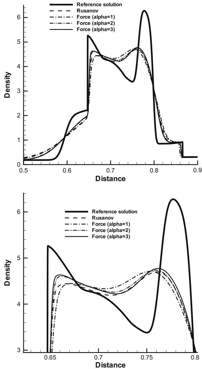
Fig. 3. Gas density for the 1D two-interactive blast waves problem to compare first-order Rusanov and FORCE- \alpha fluxes ( \alpha = 1, 2, 3 ) with 500 cells in [0, 1] . Reference solution obtained using Godunov flux with exact Riemann solver with 10,000 cells in [0, 1] . Output time t_{out} = 0.0384 . The figure below is a zoom of the figure on top.
