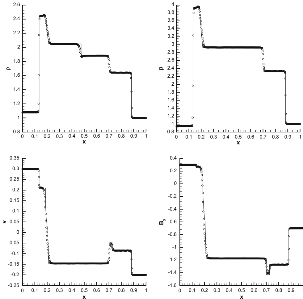
Fig. 8. Results for the RMHD Riemann problem 2 at t = 0.55 computed in 2D on 17,628 triangles. P_0P_2 WENO scheme (circles) and exact reference solution [15].
