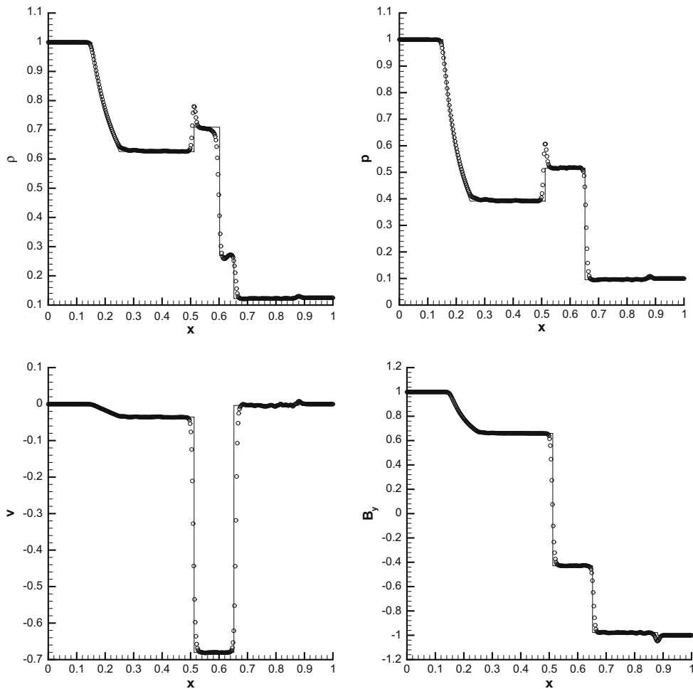
Fig. 7. Results for the RMHD Riemann problem 1 at t = 0.4 computed in 2D on 17,628 triangles. P_0P_2 WENO scheme (circles) and exact reference solution [15].
